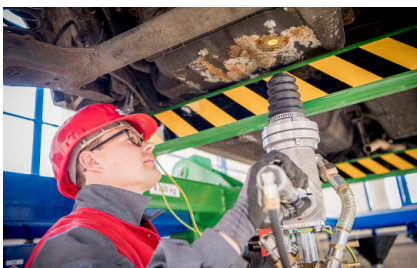
Heavy Duty Tank Drilling Machine
